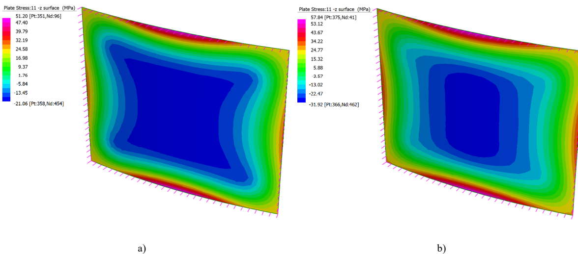
Fig. 4a, b) Maximum principal stresses of the cylindrically curved panel using linear analysis (51.20MPa) and nonlinear geometry analysis (57.84MPa)
